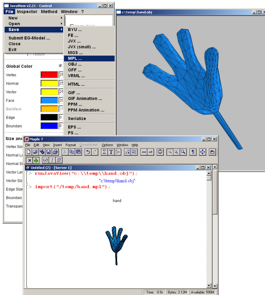
Fig. 6. Import a wealth of 3D file formats into Maple via JavaView's geometry loaders. For example, OBJ is the standard file format of Java3D and Wavefront, and accepted by rendering software like Maya.
