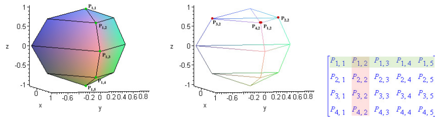
Fig. 3. Polyhedral meshes in the Maple Plot data structure.
