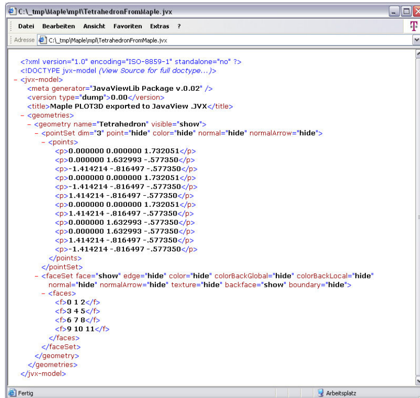
Fig. 11. View a Maple plot as formatted XML document, and collapse and expand individual parts of the markup tree. The JVL command runMarkupTree makes use of JavaView's JVX file format and the formatting capabilities of the Internet Explorer. Here the vertices and faces of a tetrahedron are displayed.
